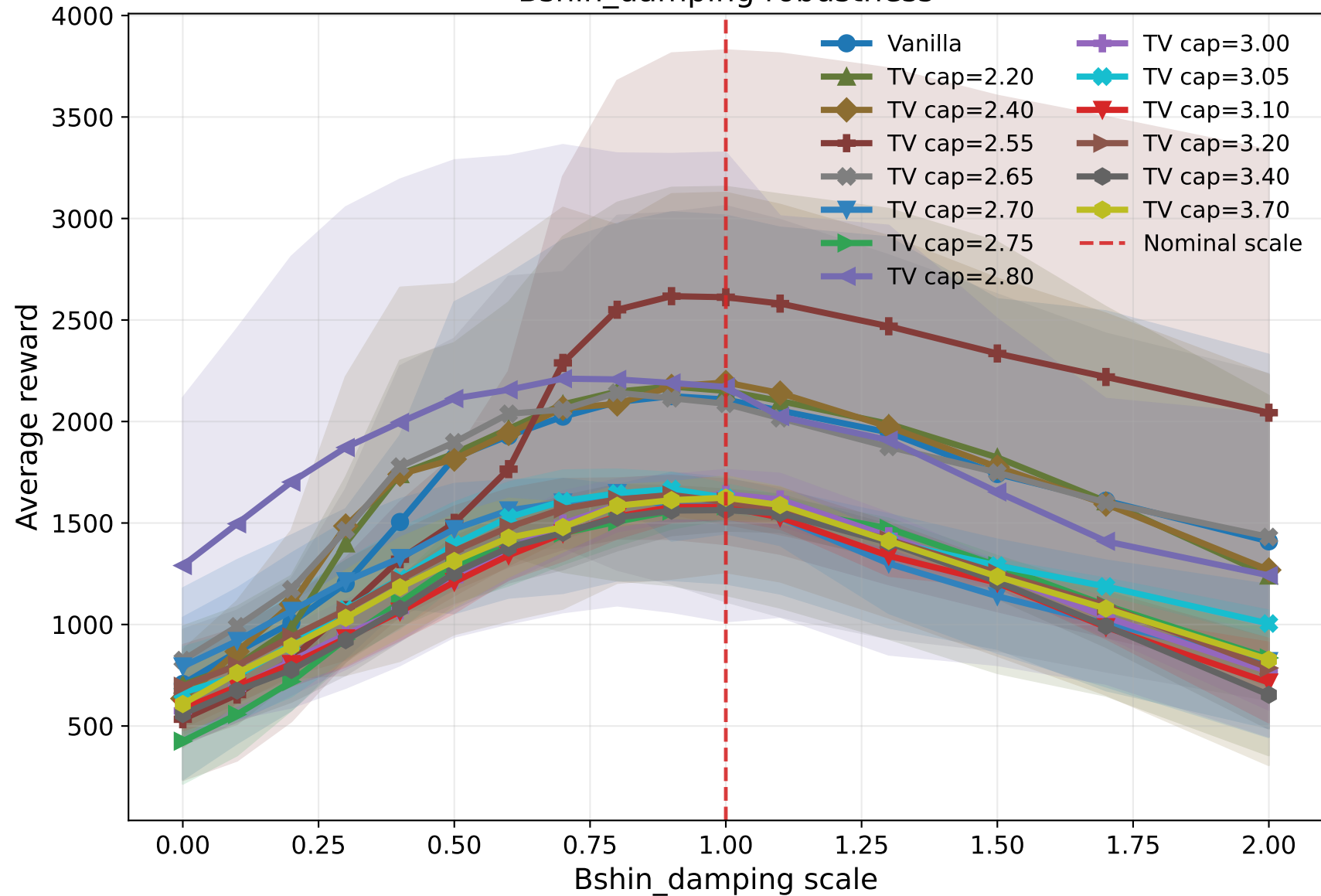
Bshin_damping robustness
